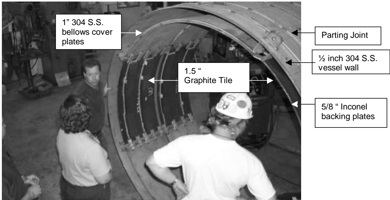
Figure 6 Vacuum vessel surrogate prior to filling
