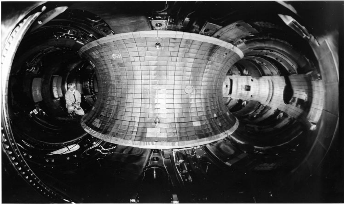
Figure 1 Internal TFTR vessel (prior to tritium operations)
