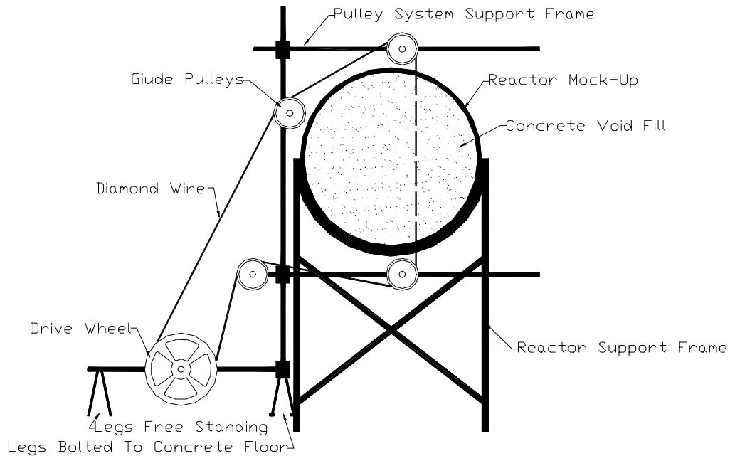
Water cooling set-up – Figure 5
