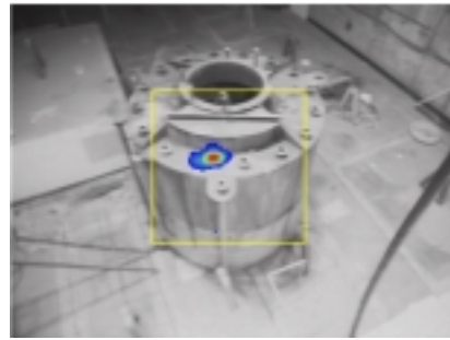
Figure 3 Gamma Image #4 obtained for the High Rad Tank on cell 35
