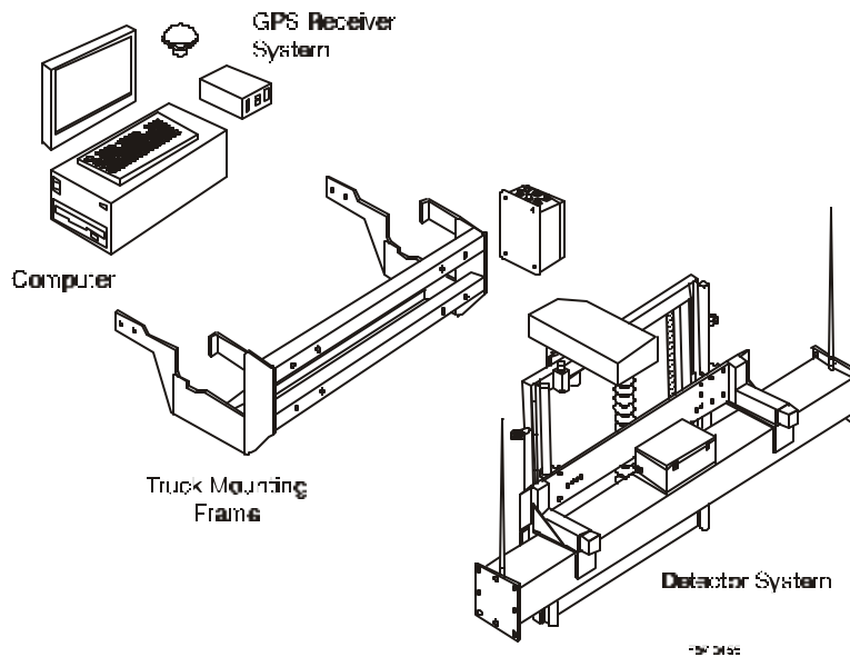
Figure 5. The framework of the GPRS system used at the INEEL.
