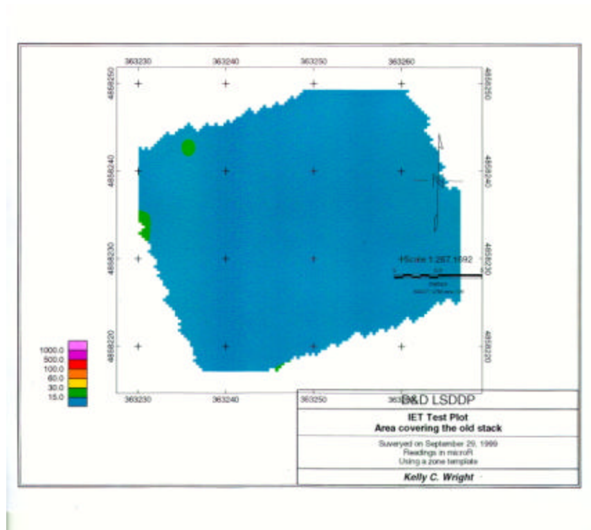
Figure 4. Graphical display of the GPRS survey result from IET stack trench.
