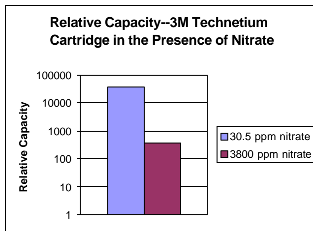
Figure 3. Relative capacity of 3M technetium cartridge in the presence of nitrate.
