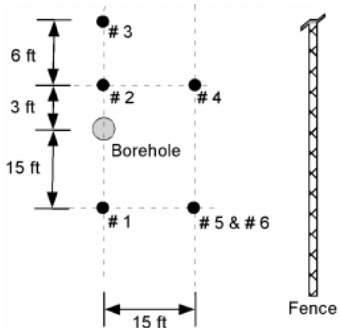
. Location of CPT penetrations with respect to past soil boring.
