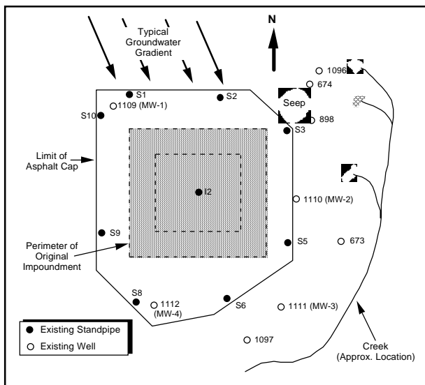
Figure 8. Pre-barrier site plan
