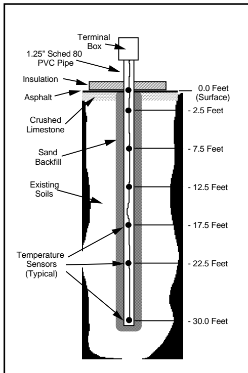
Figure 7. Typical temperature monitoring well
