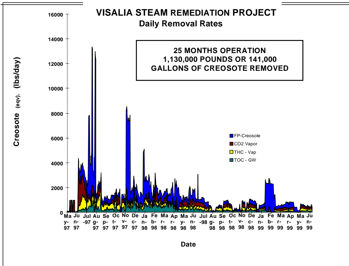
Figure 6. Daily Removal Rates at the Visalia Steam Remediation Project
