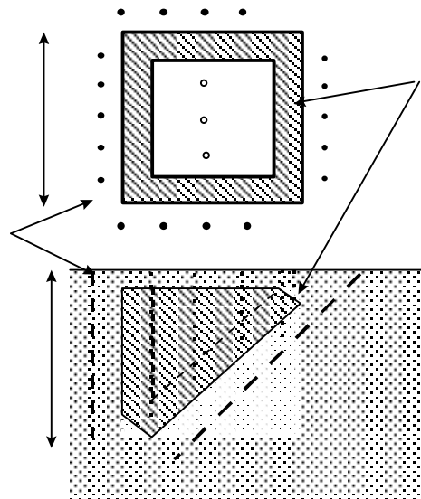
Figure 10. Schematic of the BNL barrier and the SEAttrace™ monitoring array configuration at the Viscous Liquid Barrier (VLB) test site in Brookhaven, NY. Top view of Barrier and side view of slant side wall.
