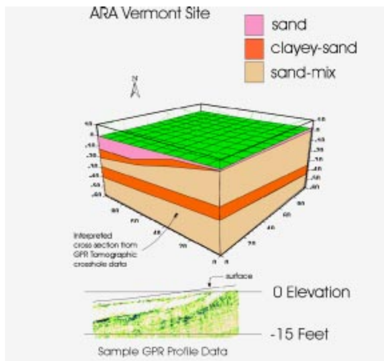
Figure 8. 3D map of major subsurface layers.
