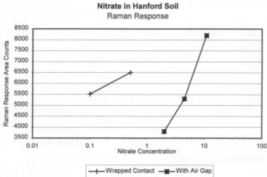
Figure 4. Nitrate concentrations (wt %) in Hanford soil.
