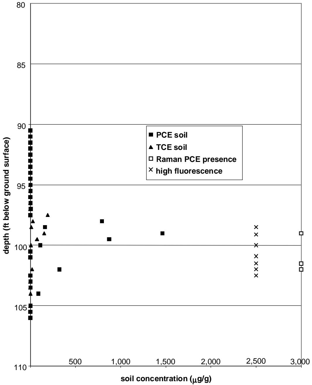
Figure 5. Raman and fluorescence vs soil concentrations (M Area Basin).
