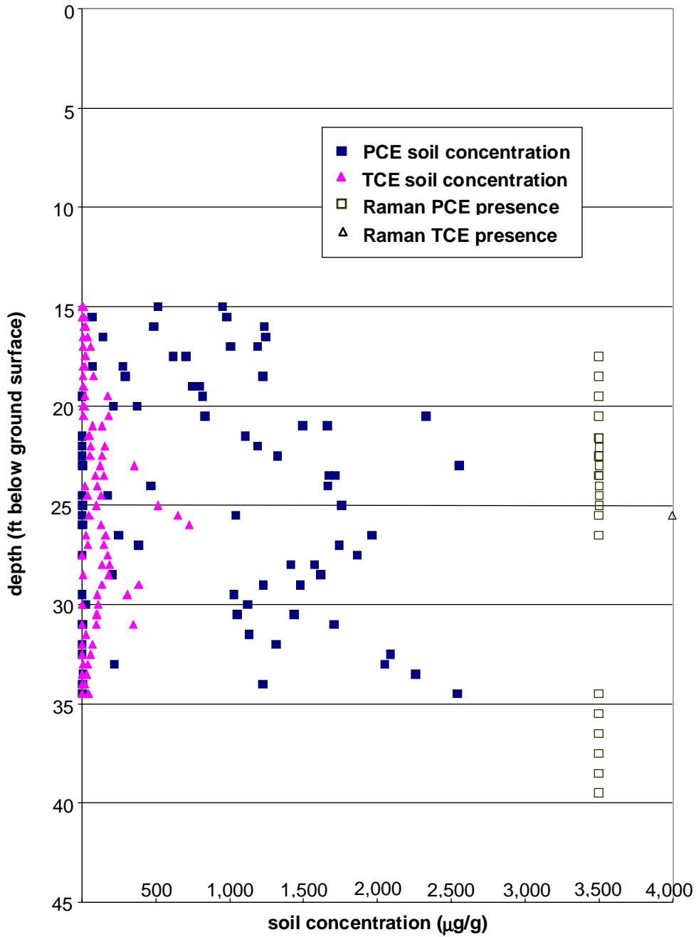
Figure 6. Raman vs soil concentrations (321-M Solvent Storage Tank).
