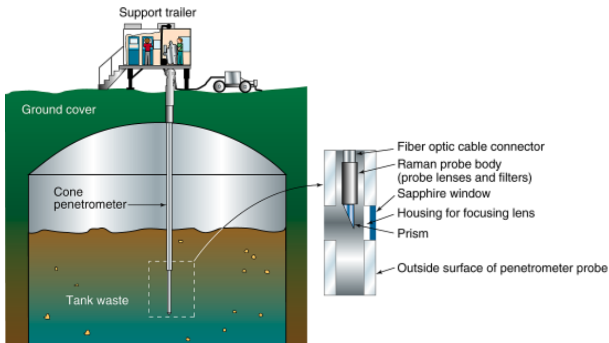
Figure 1. Raman probe deployed by a cone penetrometer inside an underground storage tank.
