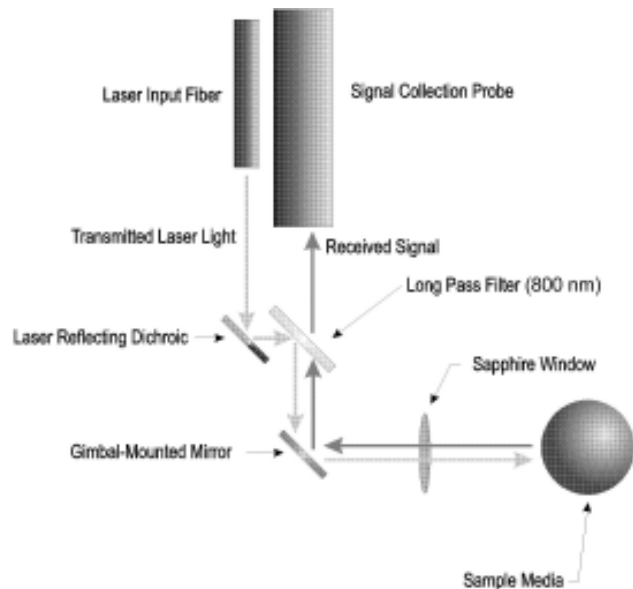
Figure 2. Raman probe operation.
