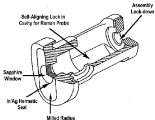
Figure 3. Sapphire window assembly.
